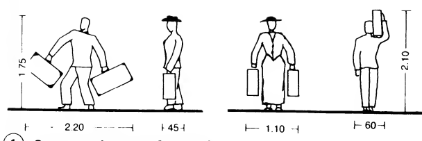
1 Space requirements for people
